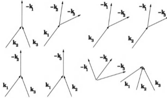
Figure 3: Diagrams for three phonon processes: for example the top-left diagram represents \hat{a}_{-k_1 j_1}^\dagger \hat{a}_{k_2 j_2} \hat{a}_{k_3 j_3} . Figure from [20, p.175].
